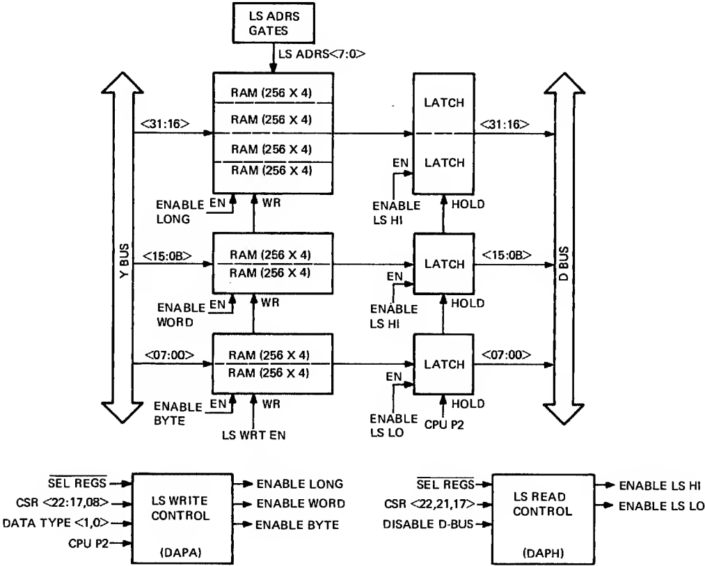
Figure 6-10 Local Store Configuration
